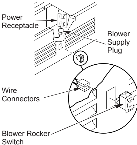
Figure 5: Connecting Switch and Supply plug
