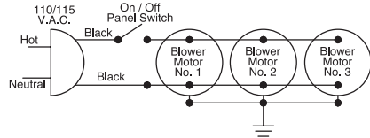
Figure 6: Wiring Diagram
