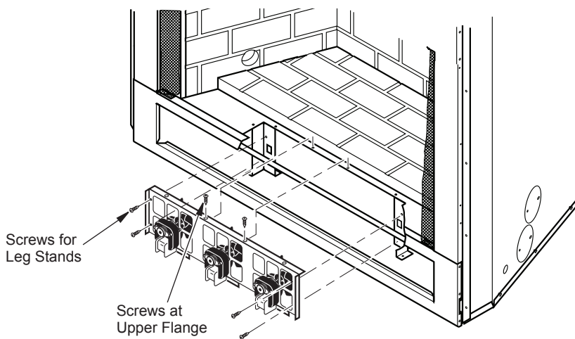
Figure 4: Mounting BK3 Blower
