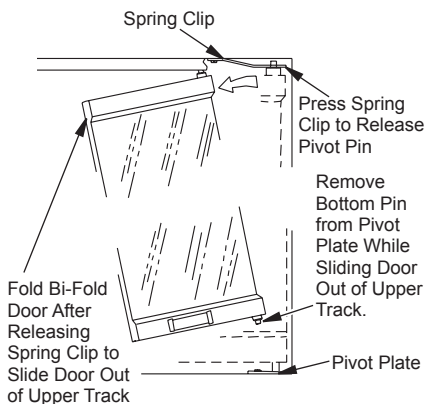
Figure 2: Removing Glass Doors
