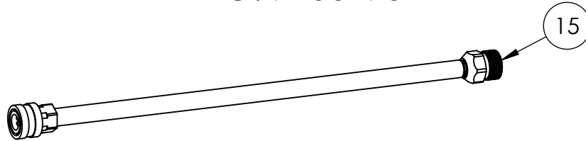
LANCE, 16" W/ 1/4"QC(F) x M22(M) PART NO. 7103550
