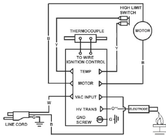
CONNECTION DIAGRAM
