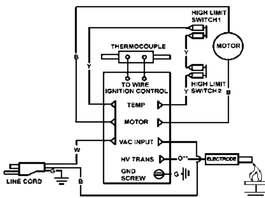
CONNECTION DIAGRAM
