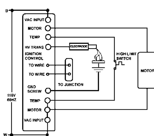
SCHEMATIC DIAGRAM
