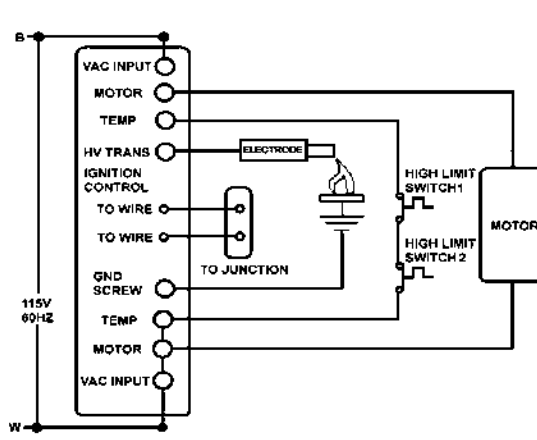
SCHEMATIC DIAGRAM
