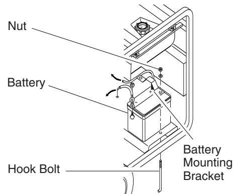
Figure 11 - Battery Hold-Down System (Model MGH10000 Shown)
