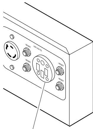
Figure 15 - Receptacle Locations
