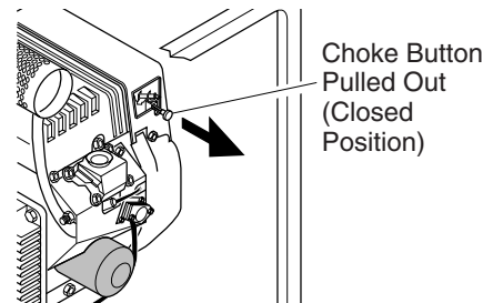
Figure 19 - Choke Button Closed (Model MGH10000 Only)
