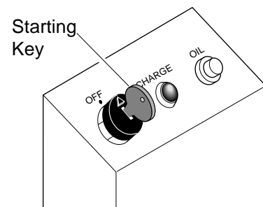
Figure 18 - Starting Key
