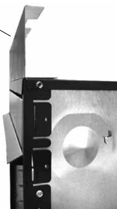
Drywall Backstops (bent up for 1/2" or 5/8")
