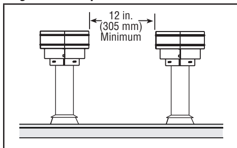
Figure 4: Multiple Terminations
