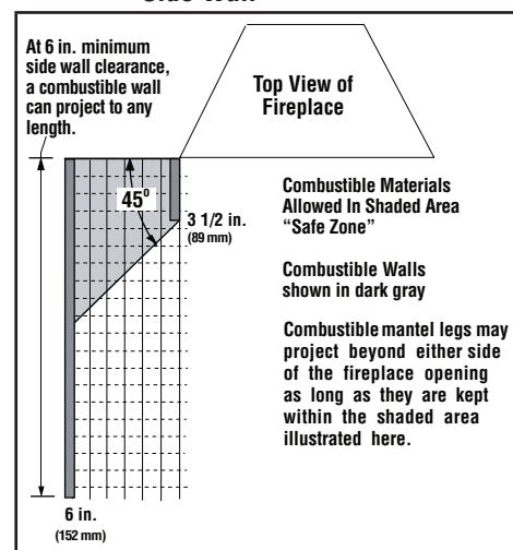
Figure 9: Minimum Distance to Side Wall
