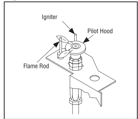
Figure 40: Electronic Pilot
