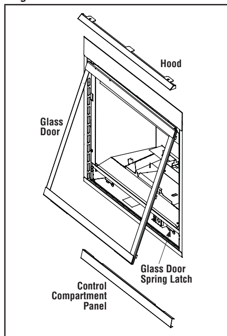
Figure 33: Glass Door
