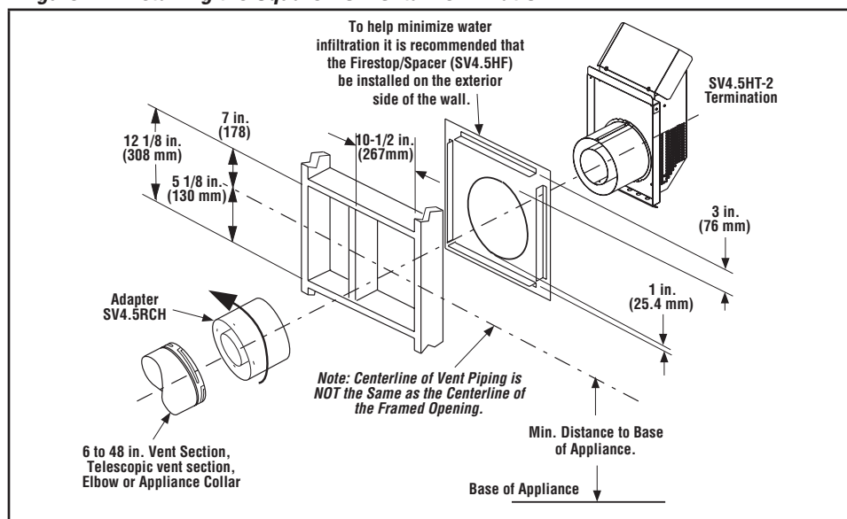
Figure 22: Installing the Square Horizontal Termination
