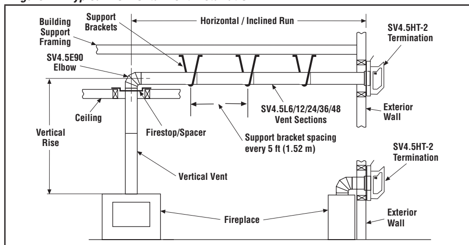
Figure 21: Typical Horizontal Vent Installation
