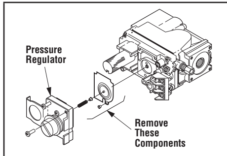
Figure 37: Millivolt Valve Regulator Conversion
