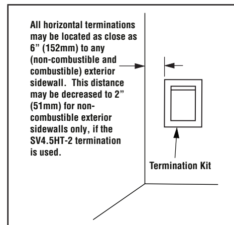
Figure 7: Horizontal Vent Termination Clearances
