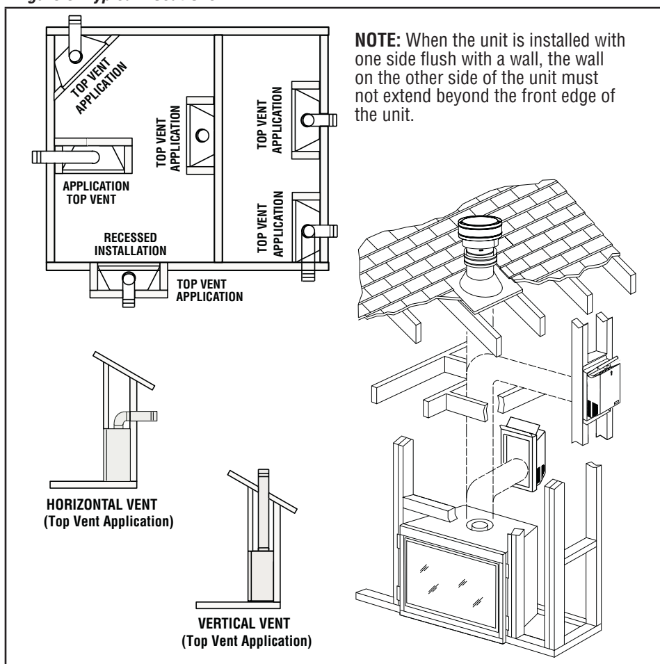
Figure 3: Typical Locations
