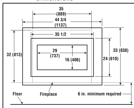
Figure 36: Contemporary Façade Dimensions
