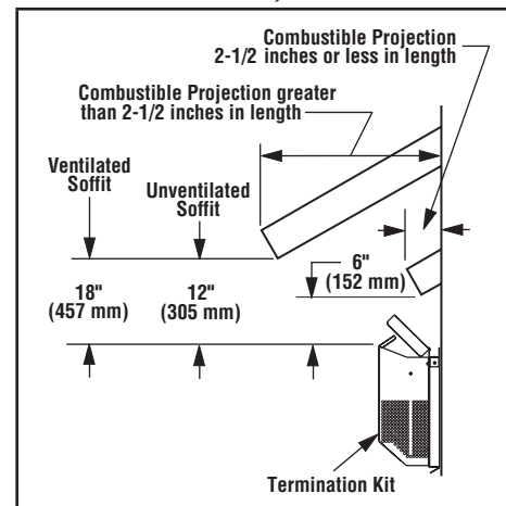
Figure 6: Horizontal Vent Termination Clearances, Side Elevation
