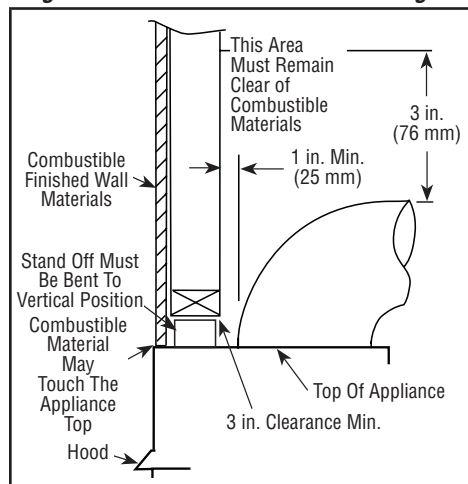
Figure 35: Combustible Wall Framing
