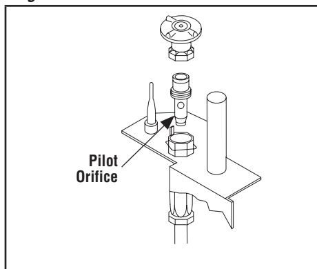
Figure 39: Millivolt Pilot
