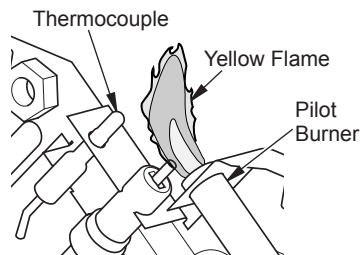
Figure 25 - Incorrect Pilot Flame Pattern BURNER FLAME PATTERN
