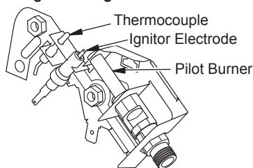
Figure 23 - Pilot (actual pilot may vary)
