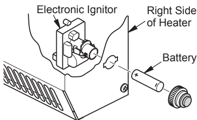
Figure 7 - Installing Electronic Ignitor
