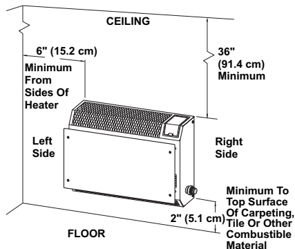
Figure 8 - Mounting Clearances As Viewed From Front of Heater
