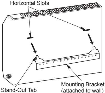
Figure 13 - Mounting Heater Onto Mounting Bracket
