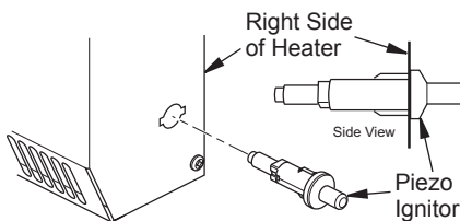
Figure 6 - Installing Piezo Ignitor
