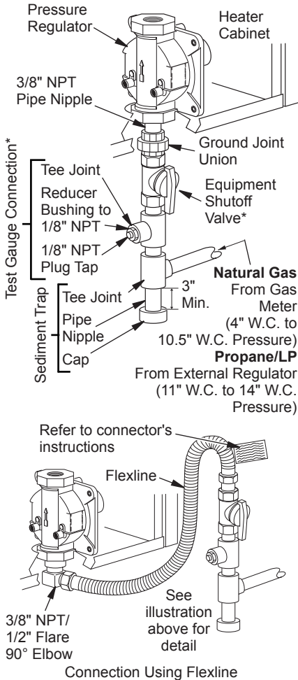
Figure 15 - Gas Connection
