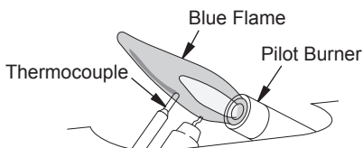
Figure 21 - Correct Pilot Flame Pattern
