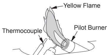
Figure 22 - Incorrect Pilot Flame Pattern
