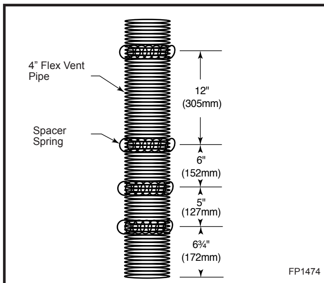
Fig. 35 Install spacer springs.
