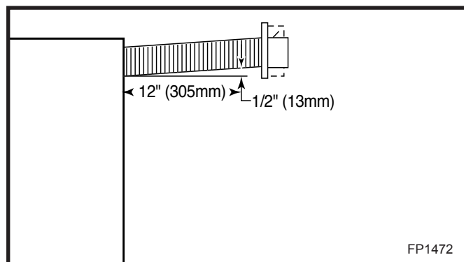
Fig. 25 There must be a 1" rise in 24" length.
