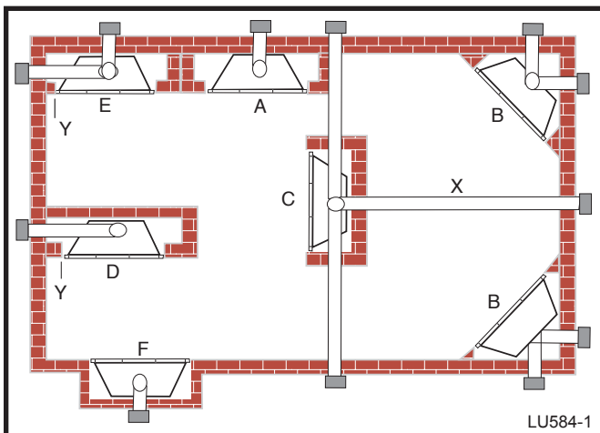
Fig. 1 Locating Gas Fireplace
