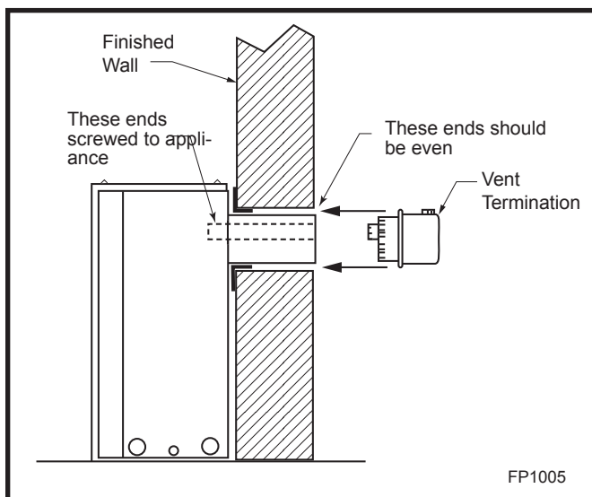
Fig. 23 Side view of final unit location, twist lock pipe.
