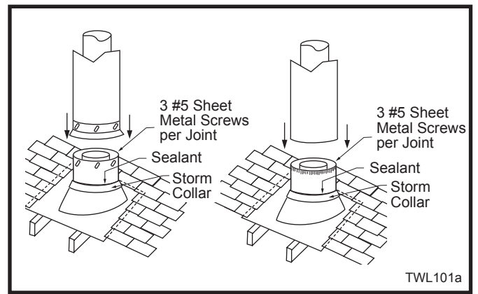
Fig. 46 Roof flashing.
