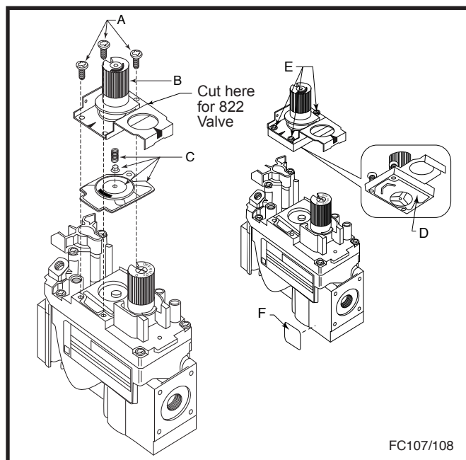
Fig. 60 Remove mounting screws, pressure regulator tower and spring and diaphragm assembly. Replace regulator.
