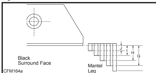
Fig. 4a Combustible mantel minimum installation.
