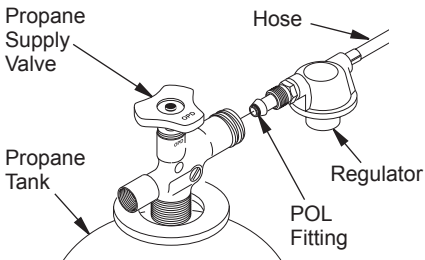
Figure 3 - Regulator Position
