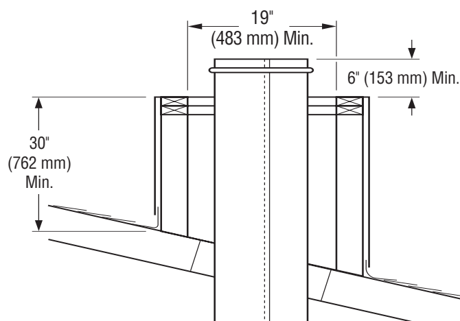
Figure 25 - Constructing Chase
