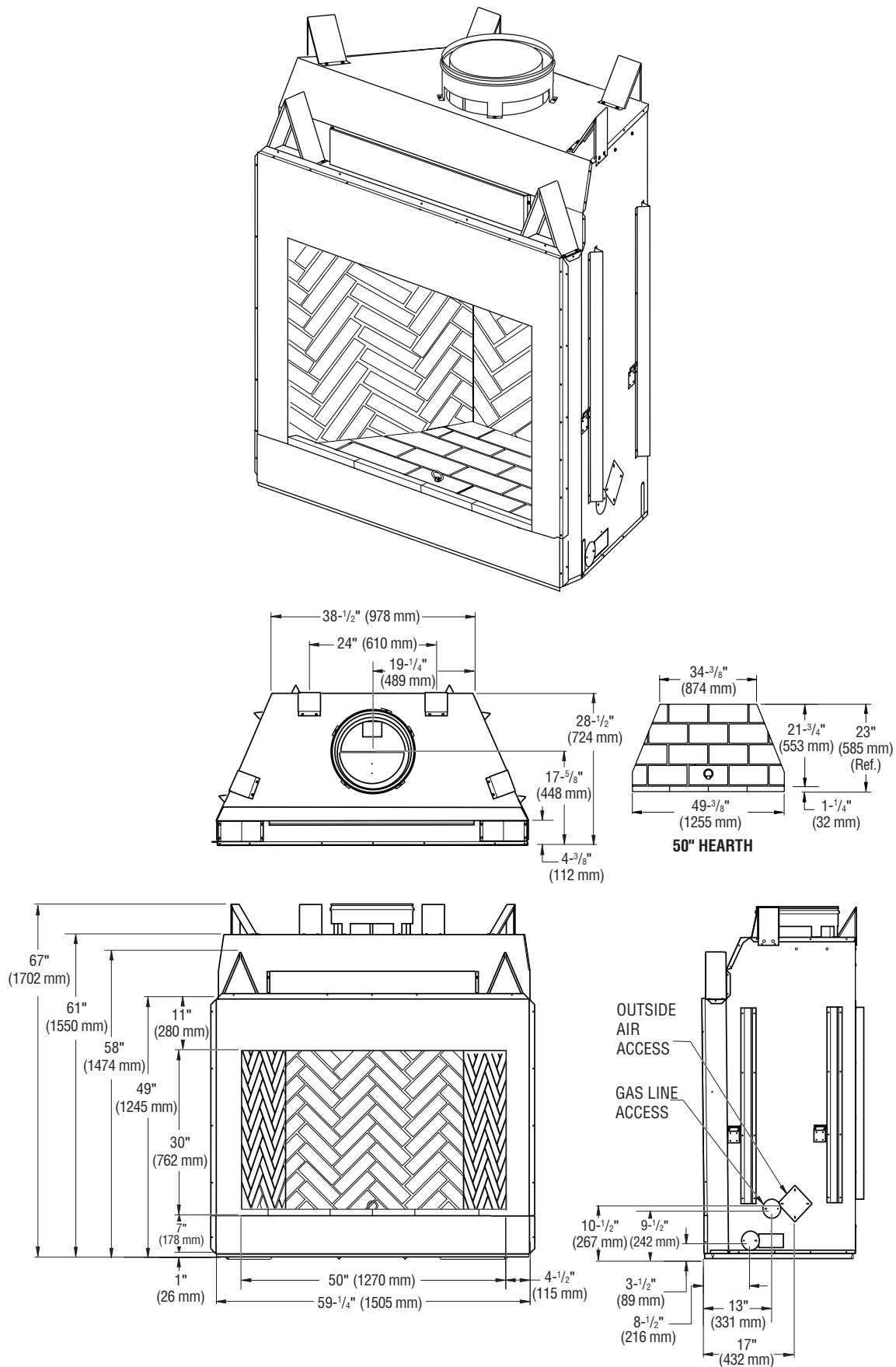
Figure 3 - 50" Models WRT6050RS, WRT6050IS, WRT6050RH and WRT6050IH
