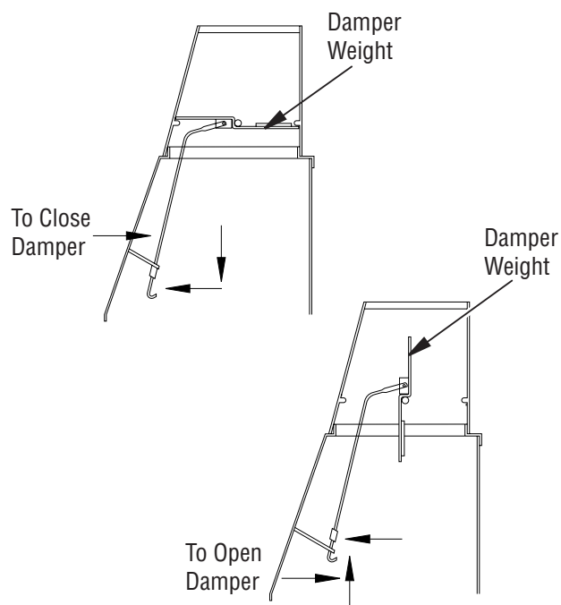
Figure 31 - Operating Damper Handle
