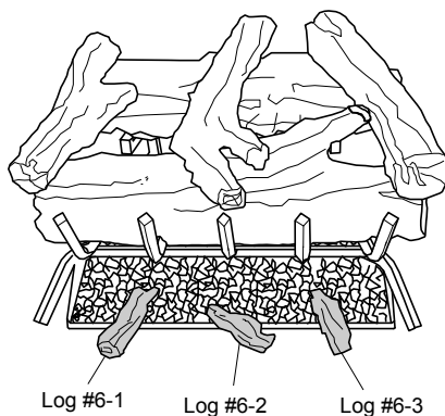
Figure 11 - Installing Logs #6-1, #6-2 & #6-3
