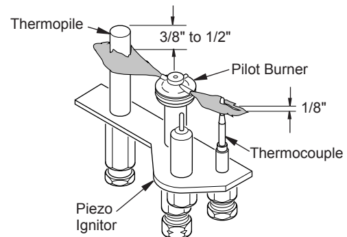
Figure 20 - Pilot Assembly
