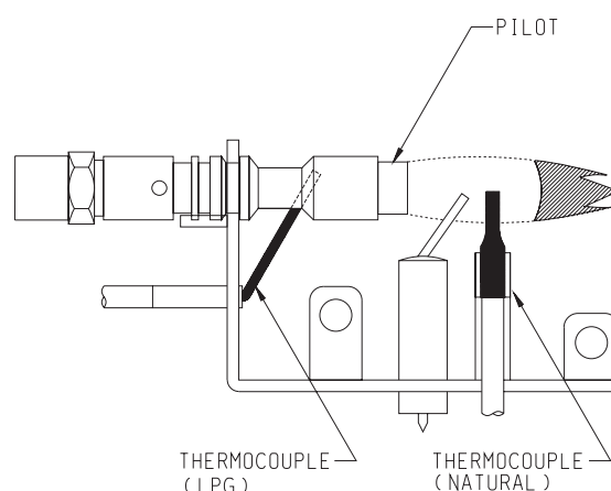
Incorrect Flame Pattern for VFDT & VFDM Figure 23
