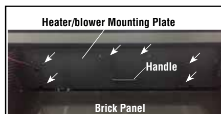
Remove screws indicated by arrows Figure 7
