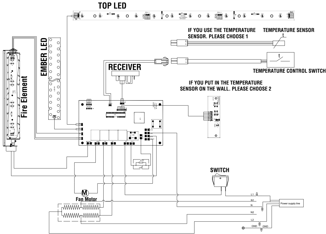
240V WIRING DIAGRAM
