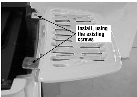
Figure 44 - Installing onto Stove Body
