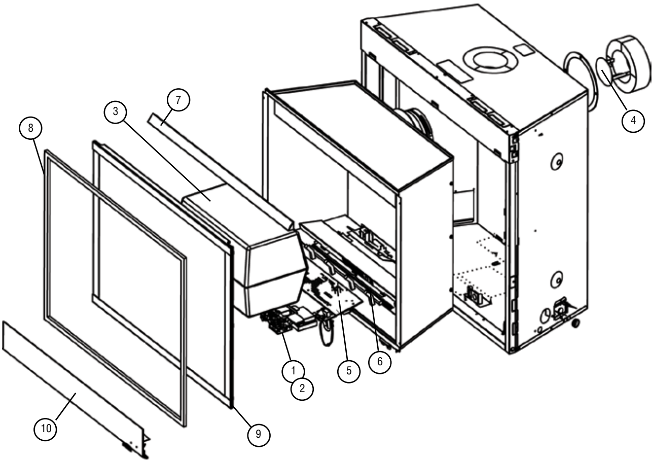
Figure 54 - Replacement Parts
