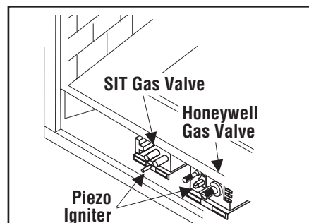
Sit and Honeywell Millivolt Gas Valve Showing Piezo Igniter Location (Each Unit is Equipped with Only One of these Gas Valves)
