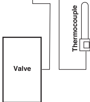
Fig. 40 Safety Limit Switch wiring.
