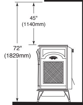
Fig. 4 Minimum ceiling clearance; minimum alcove height.
