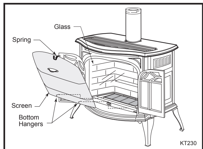
Fig. 43 Hold screen at an angle to attach bottom hangers.
