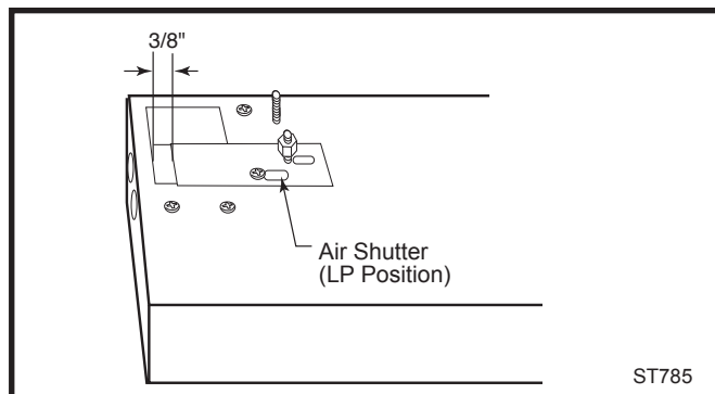
Fig. 32 LP air shutter settings.
