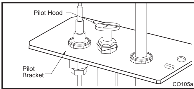
Fig. 30 Remove pilot hood.
