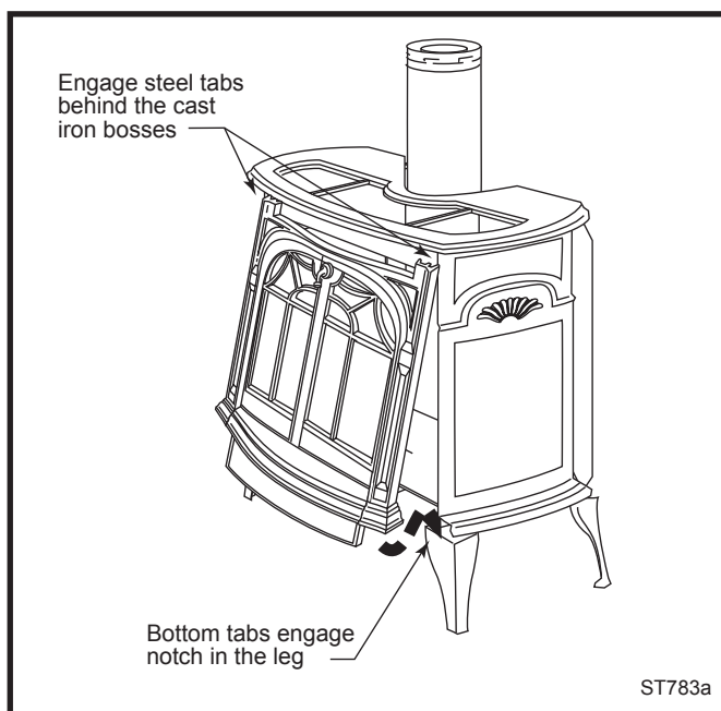
Fig. 21 Install the front plate.
