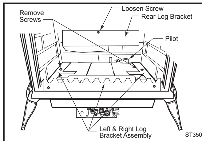
Fig. 28 Remove rear log bracket and left and right log bracket assembly.
