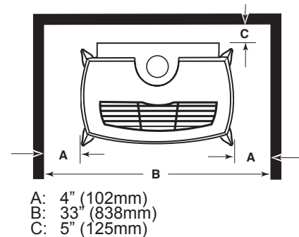
Fig. 5 The Stardance Natural Vent Stove is approved for installation into alcoves built of combustible materials.
