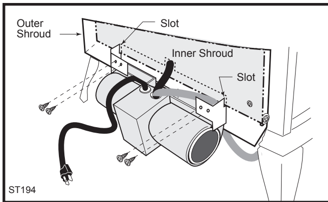
Fig. 10 Position the fan to engage the inner shroud with the fan bracket slots and secure with sheet metal screws.
