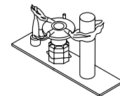
Pilot Assemblies
