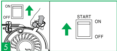
5 Place the START switch in the ON position. Pull back recoil forcefully until the engine starts.
