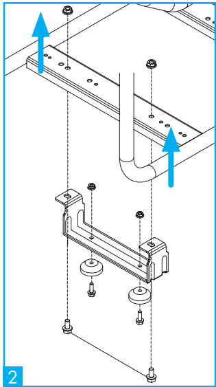
2 Install support bracket and damping feet.
