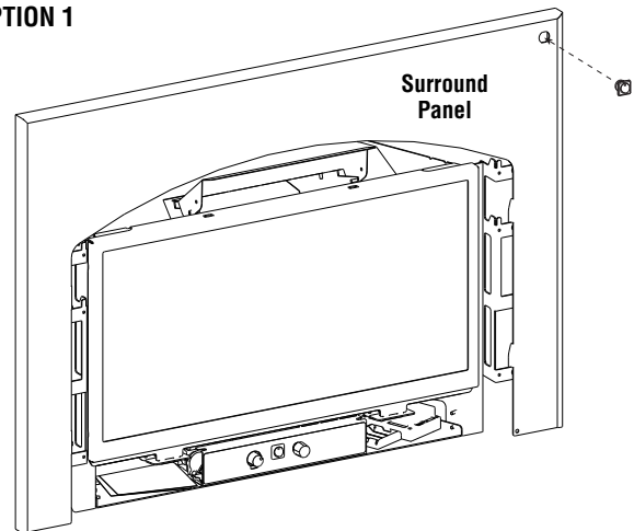
Figure 16 - Burner ON/OFF Switch On Surround
