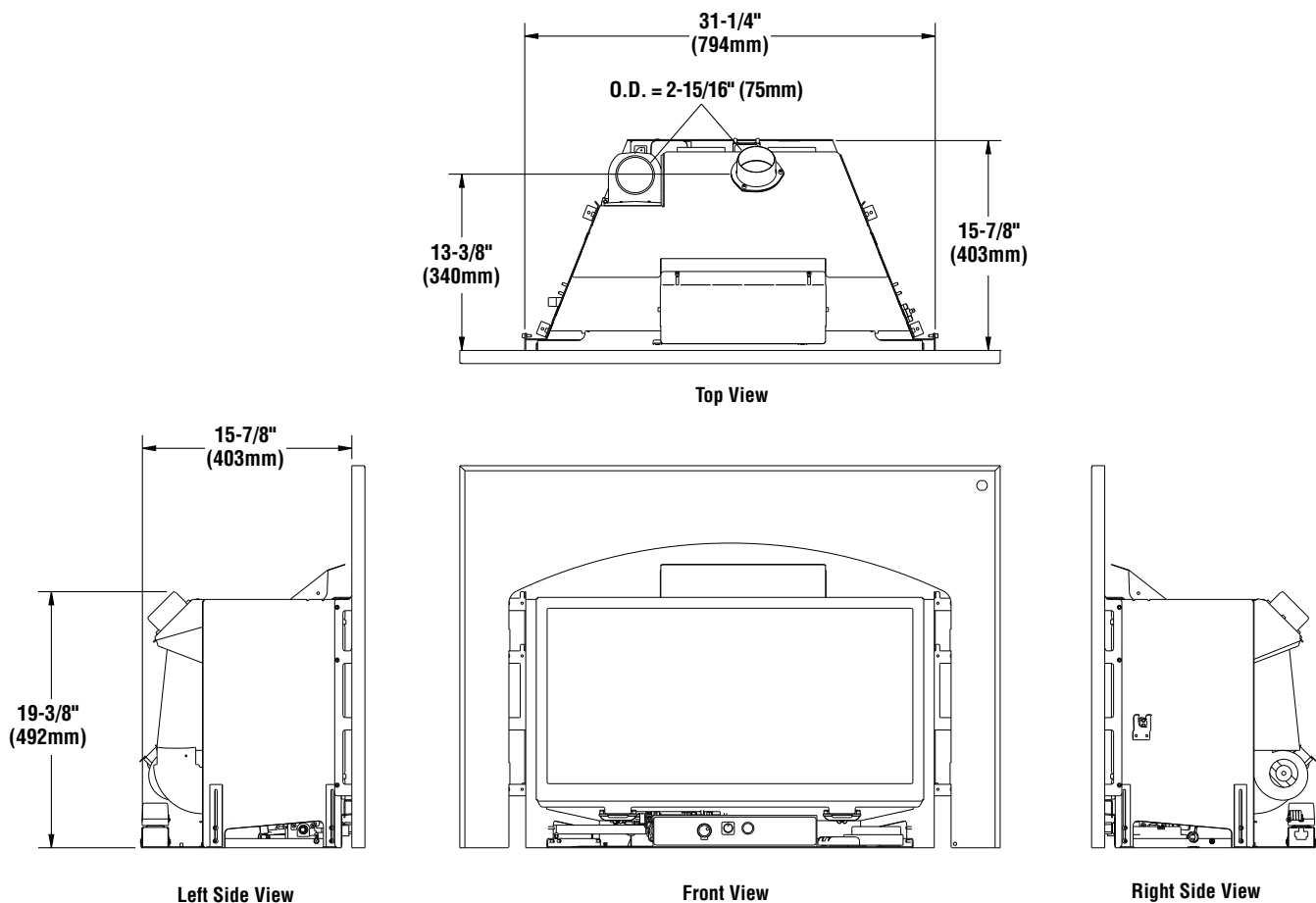
Figure 2 - Insert Dimensions
