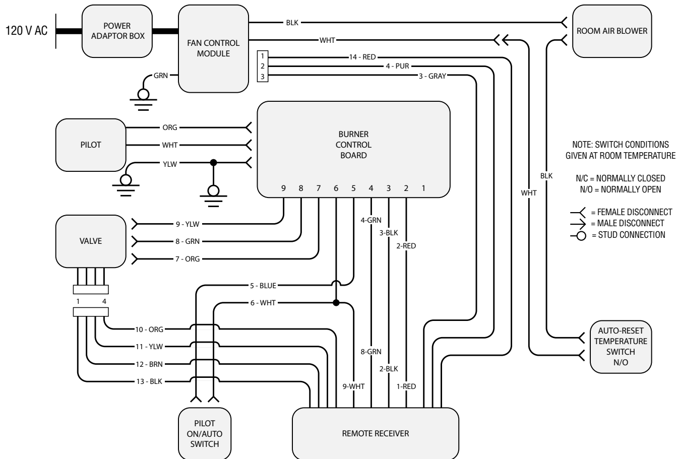
Figure 28C - Electronic Control Schematic - Models RDV33/40 TCC
