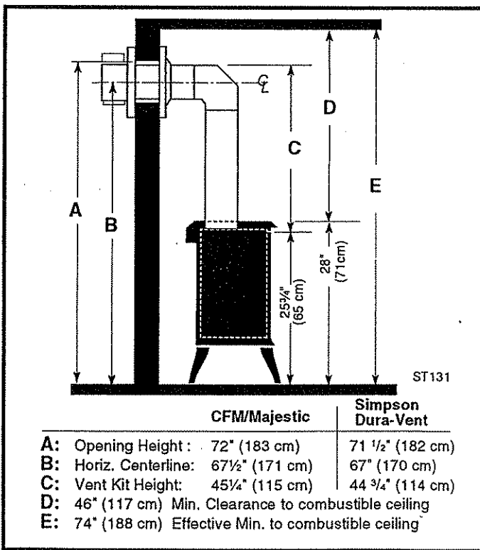
Fig. 5 Vertical dimensions for minimum vent through wall.
