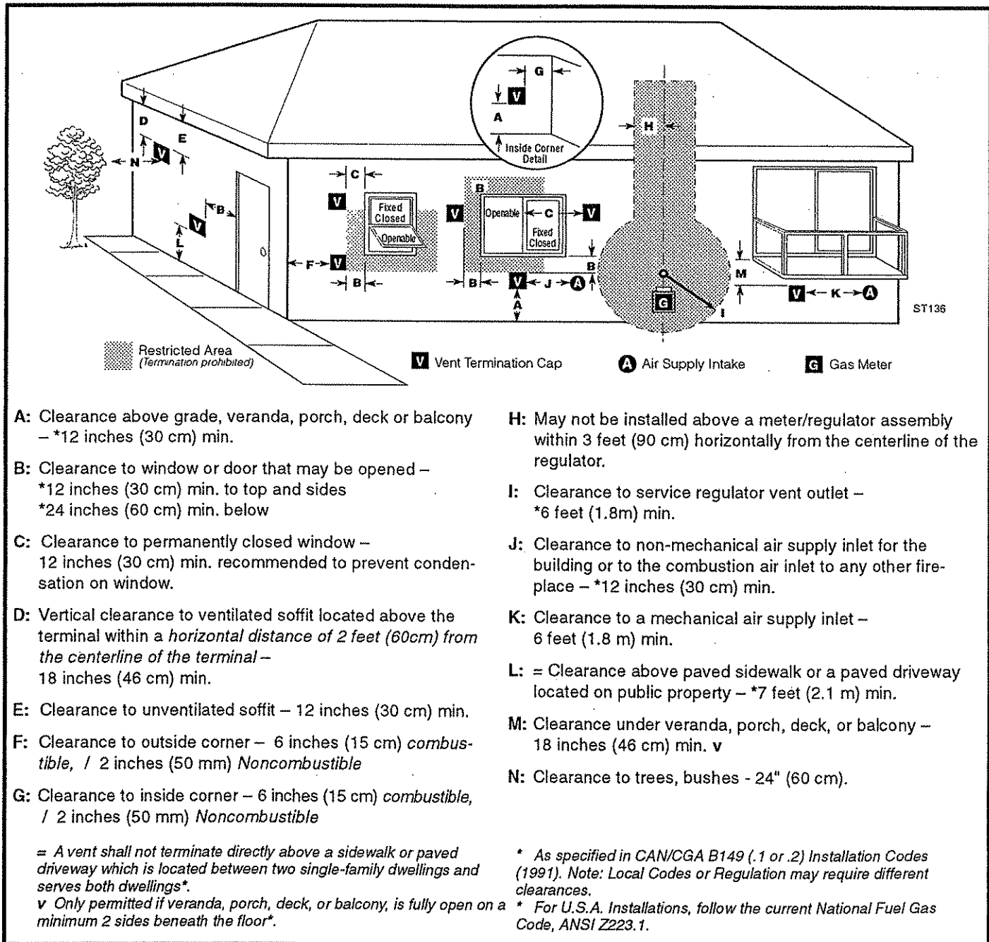
Fig. 9 Vent Termination Clearances.
