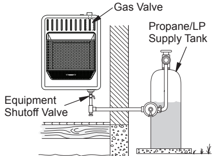
Figure 19 - Checking Gas Joints for Propane/LP Gas
