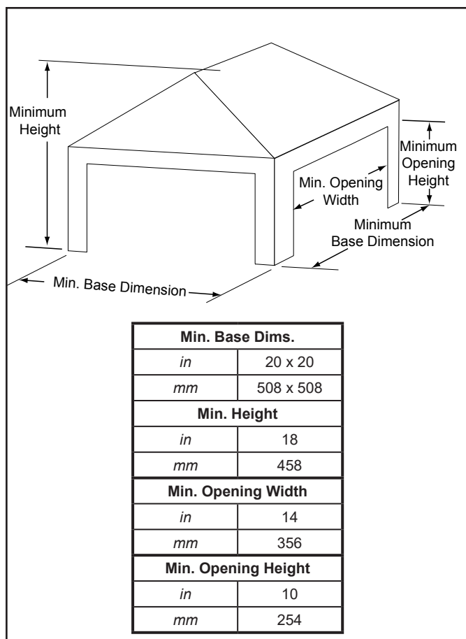
Figure 7.18 Roofed Style Shroud Dimensions
