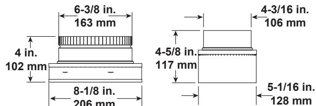
DVP-2SL Adapter
