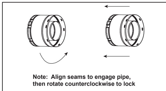
Figure 7.5 Adding Venting Components
