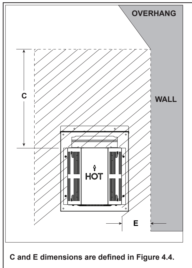
Figure 4.11 Measure Horizontal and Vertical Termination Clearance to Trapezoid Portion of Cap
