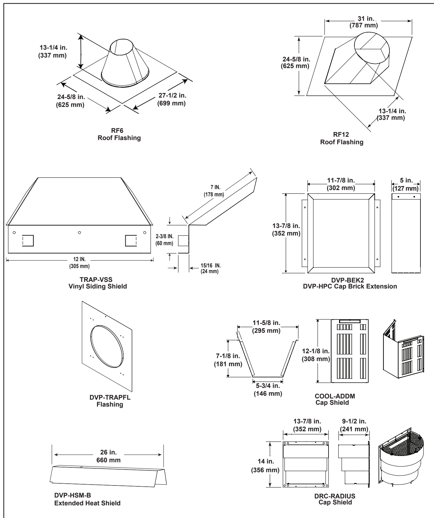
Figure 12.3 Vent Components
