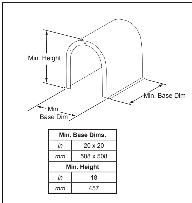
Figure 7.17 Mailbox Style Shroud Dimensions
