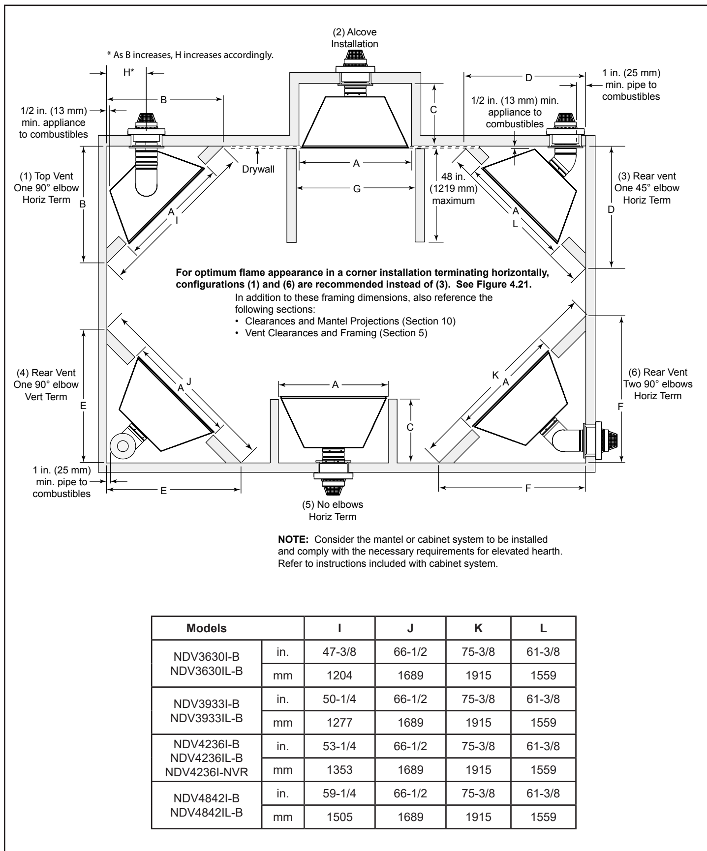
Figure 3.4 Appliance Locations - Part 2, Columns I-L
