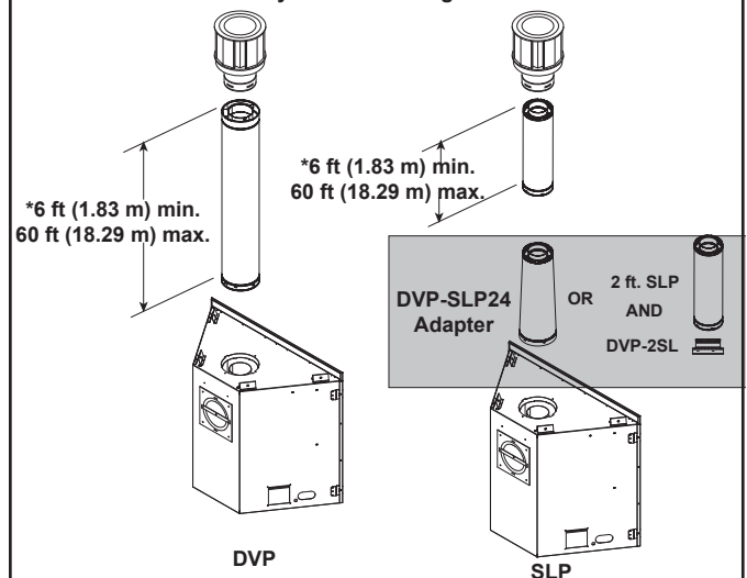
Figure 4.13 DVP-SLP24 Adapter
