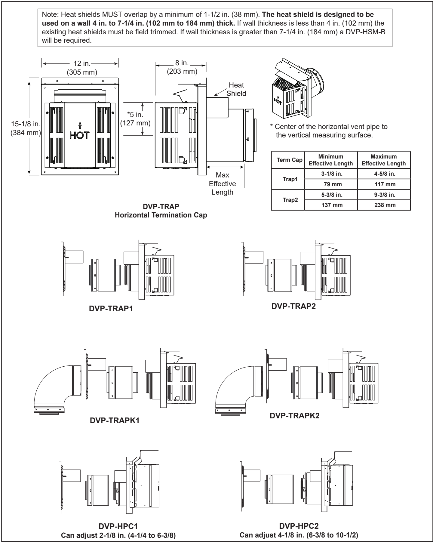
➔ Figure 12.2 DVP Vent Components
