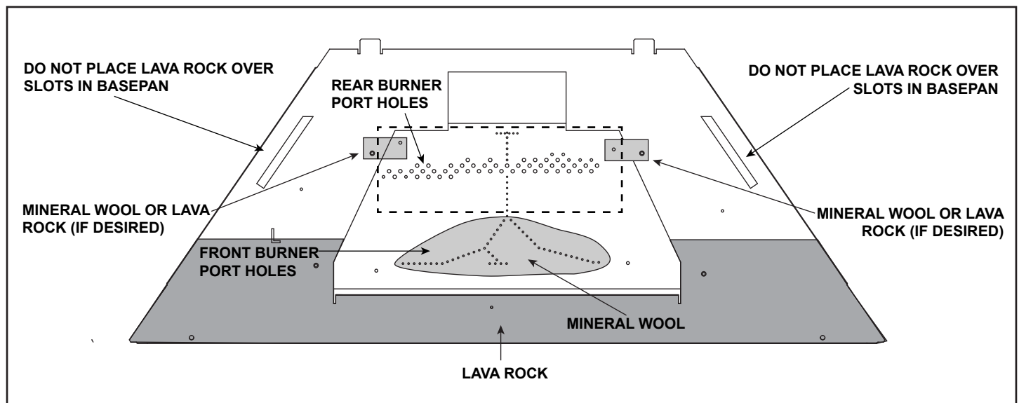
→ Figure 11.3 Placement of Mineral Wool and Lava Rock
