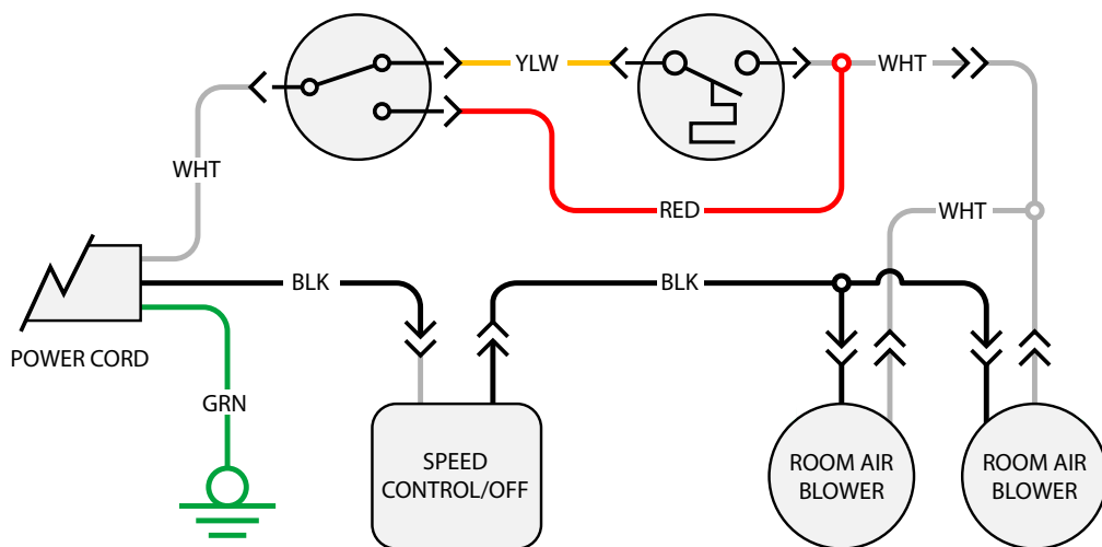
Figure 31B - ML300 Blower Wiring Schematic
