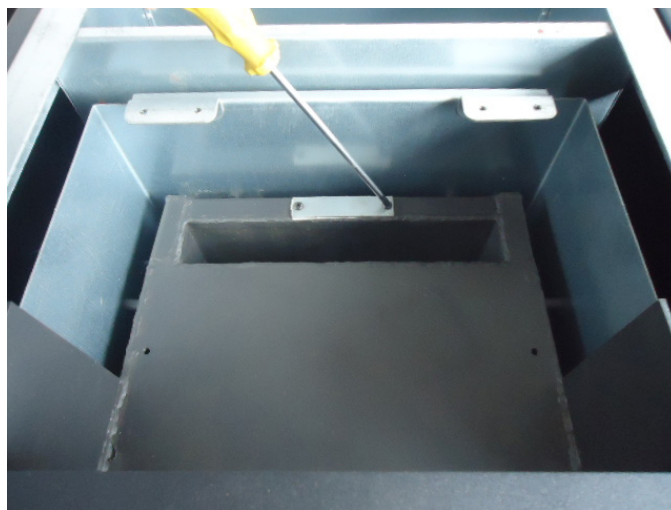
Figure 19 Outlet Duct
