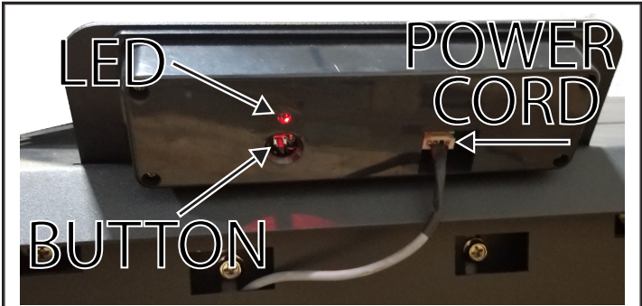
Figure 15 Display Panel Back
