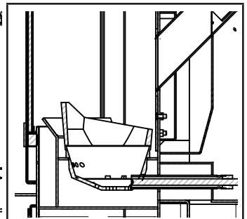
Figure 3 H3W80XL firepot
