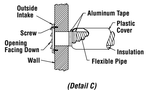
OUTSIDE AIR CONNECTION
