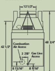
Closed End View
