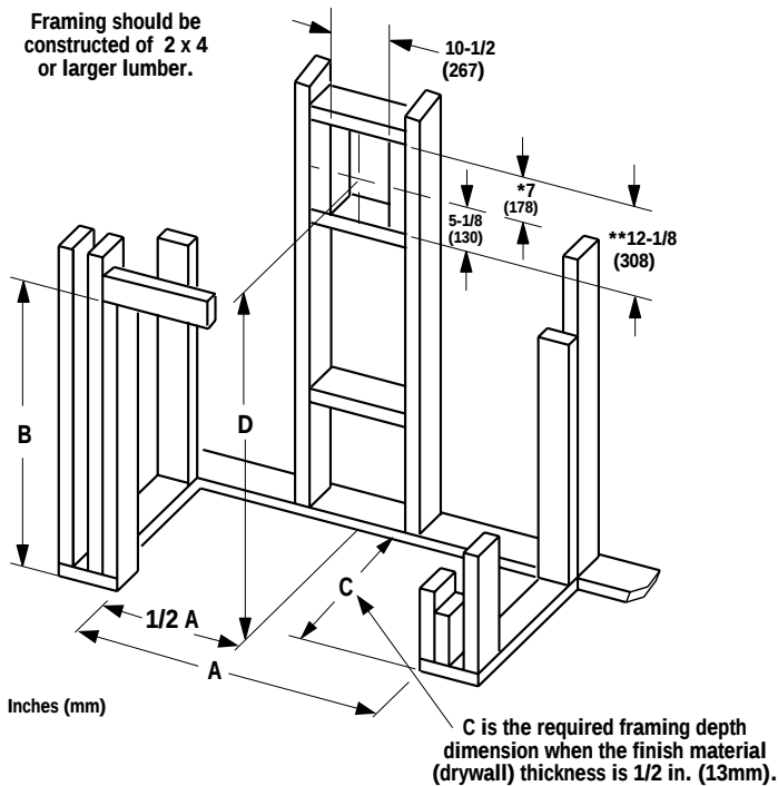
Figure 9 Framing
