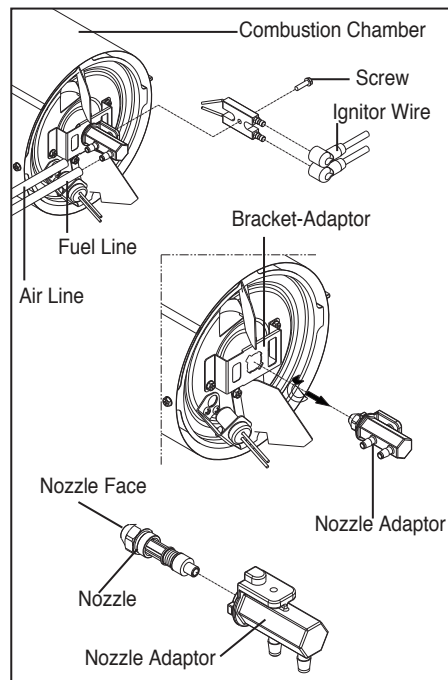
Figure 14. Nozzle Replacement
