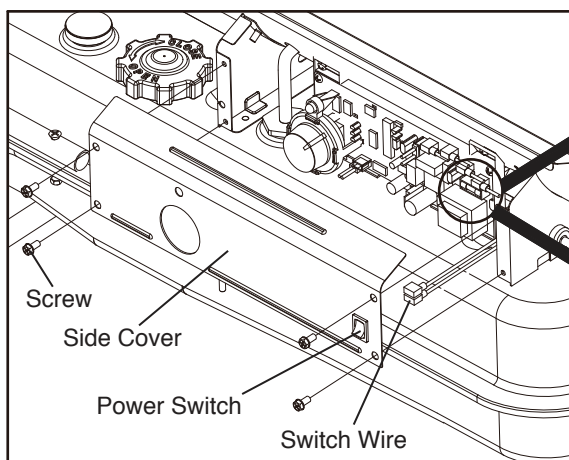
Figure 21. Replacing Fuse
