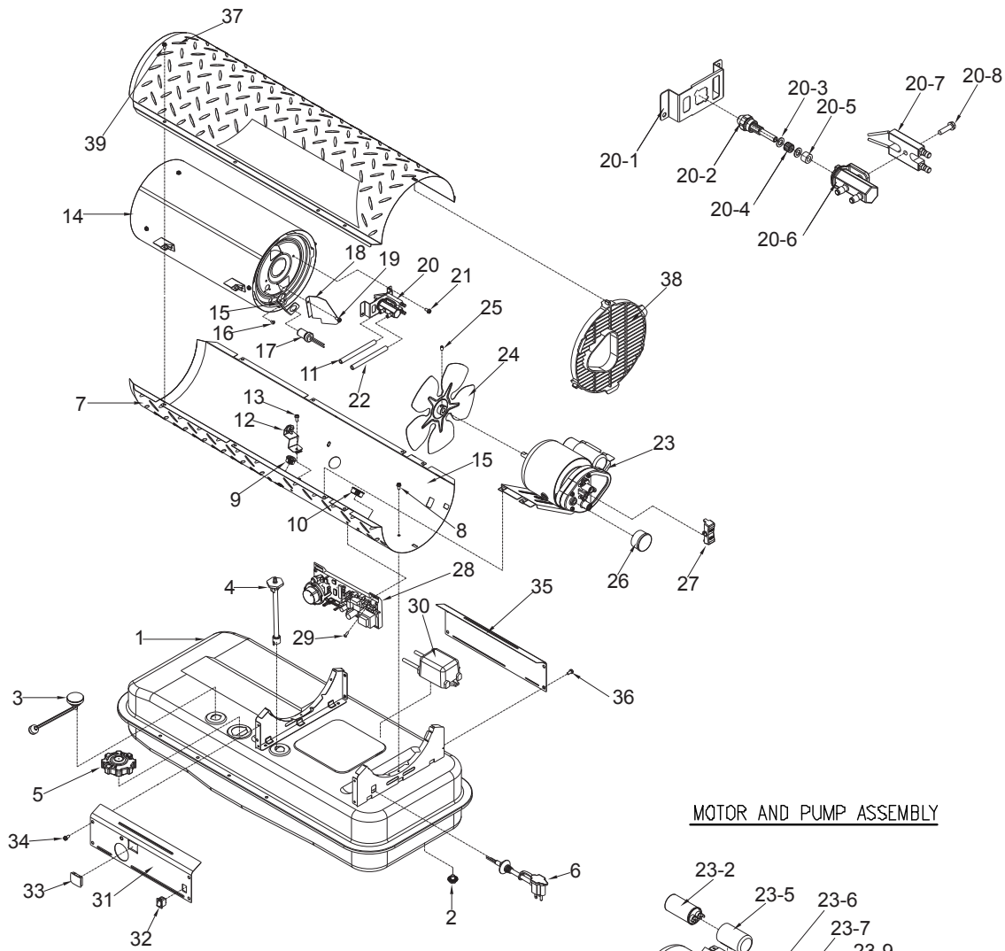
BURNER HEAD ASSEMBLY
