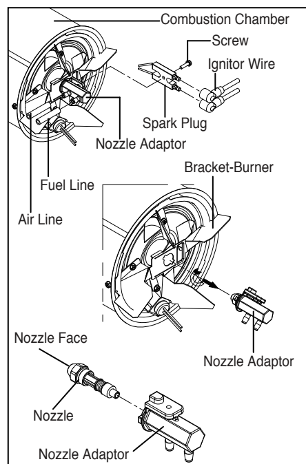
Figure 15. Nozzle Replacement
