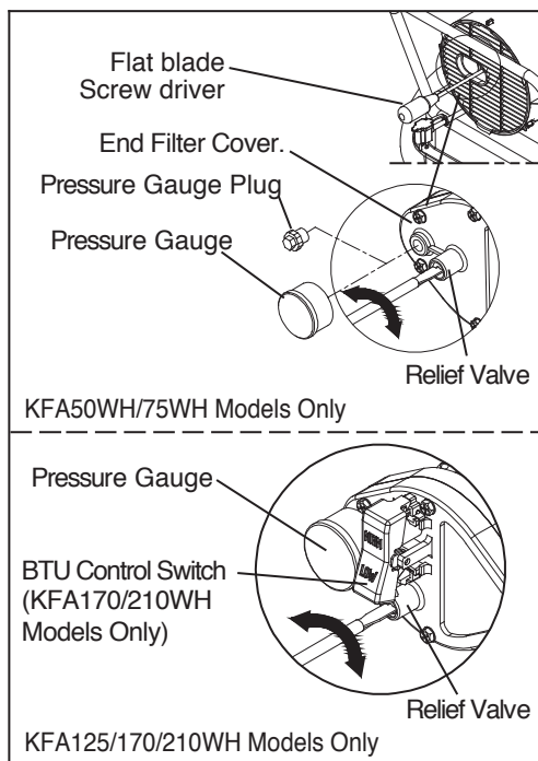
Figure 20. Adjusting Pump Pressure
