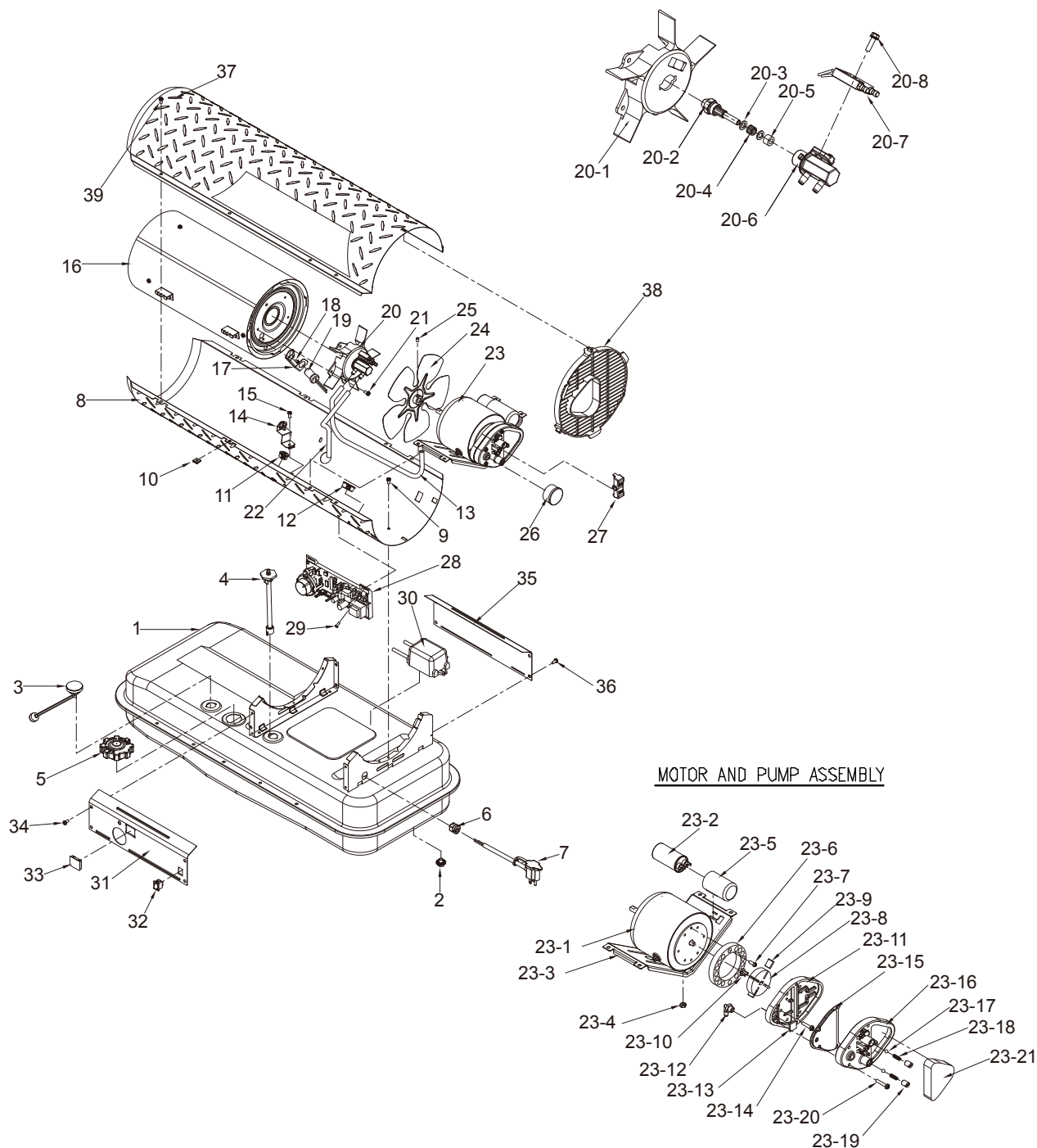
BURNER HEAD ASSEMBLY
