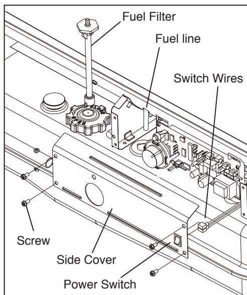
Figure 19. Fuel Filter Replacement
