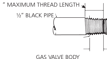
Figure 2. Gas valve connection requirements
