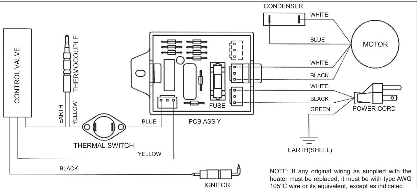
Figure 5: Wiring Diagram for Piezo/Manual Spark Models
