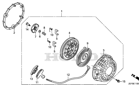
RECOIL STARTER(1)
