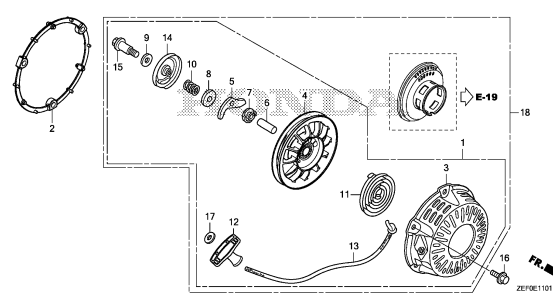
RECOIL STARTER(2)
