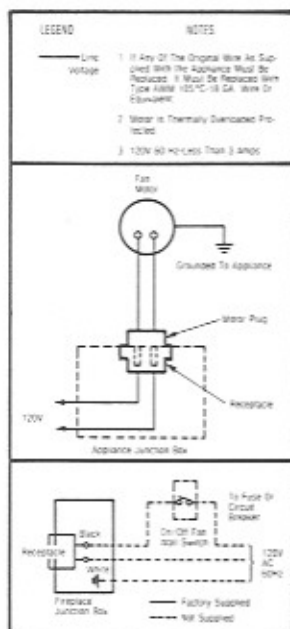
(Fan Wiring Diagram)
