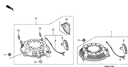
RECOIL STARTER
