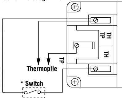
* On/off Switch, Optional Thermostat or Remote Control Receiver Figure 41
