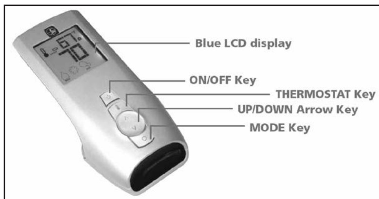
Figure 6: Proflame Transmitter.
