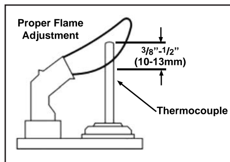
Figure 37: Proper Pilot Flame.
