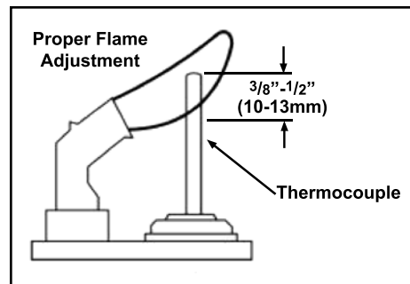
Figure 34: Proper Pilot Flame.
