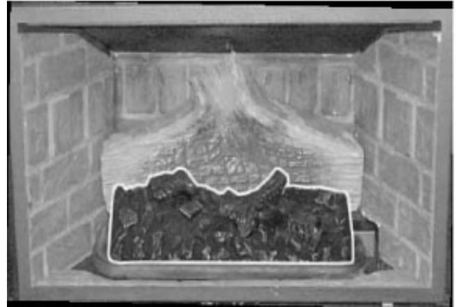
Figure 45: Place the ember bed in the center of the burner tube and pull it forward as far as it will go. Ensure it DOES NOT obstruct any part of the burner.
