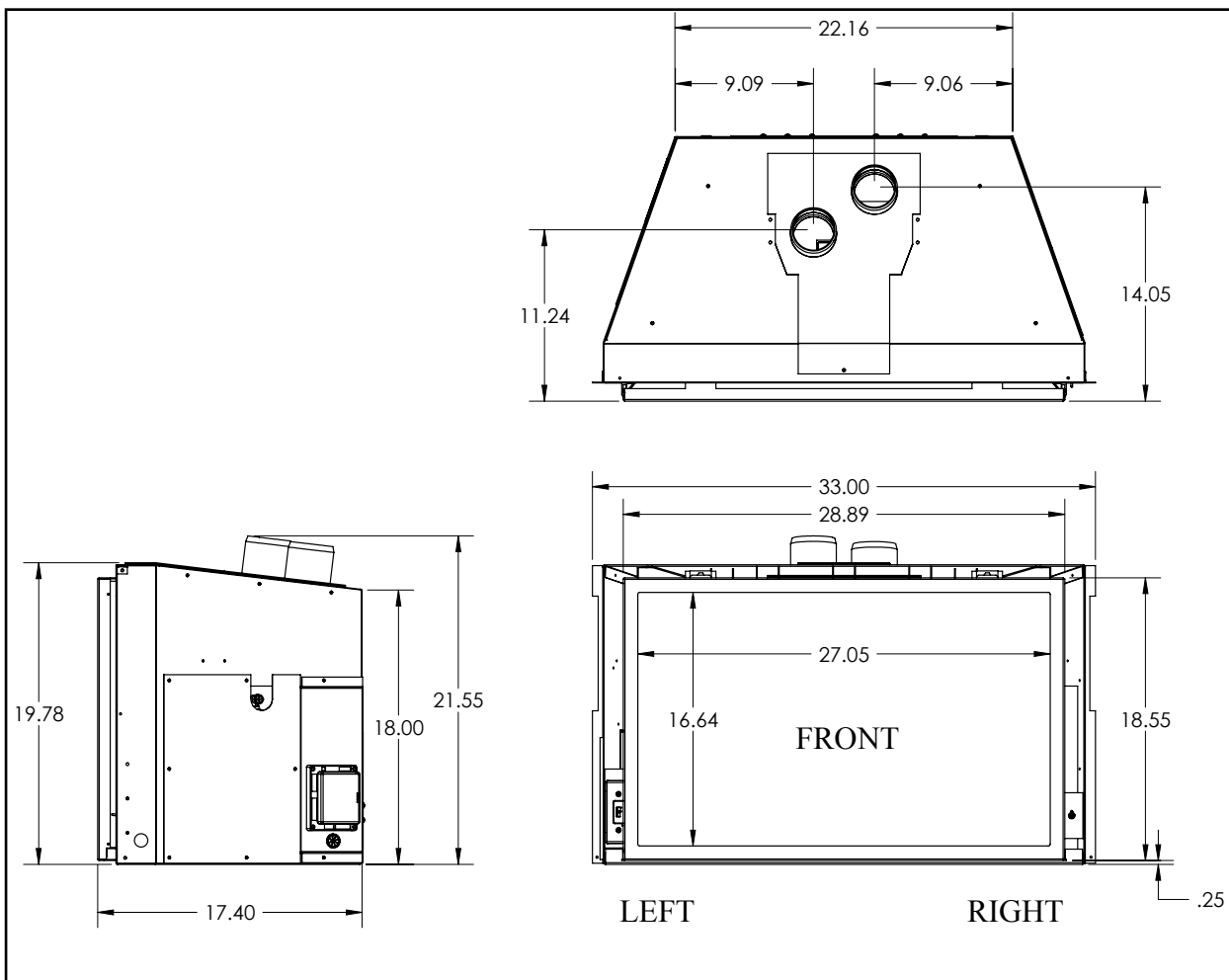
Figure 1: E33I Exterior Dimensions.
