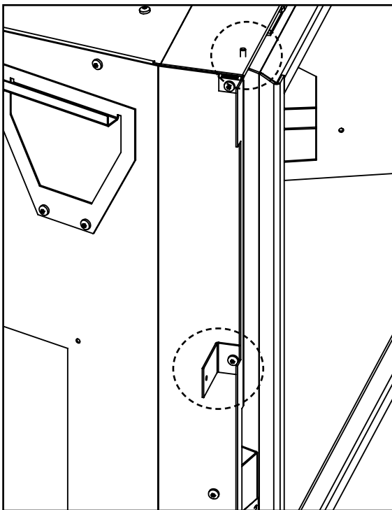
Figure 36: Panel Bracket Installed and Pin Location
