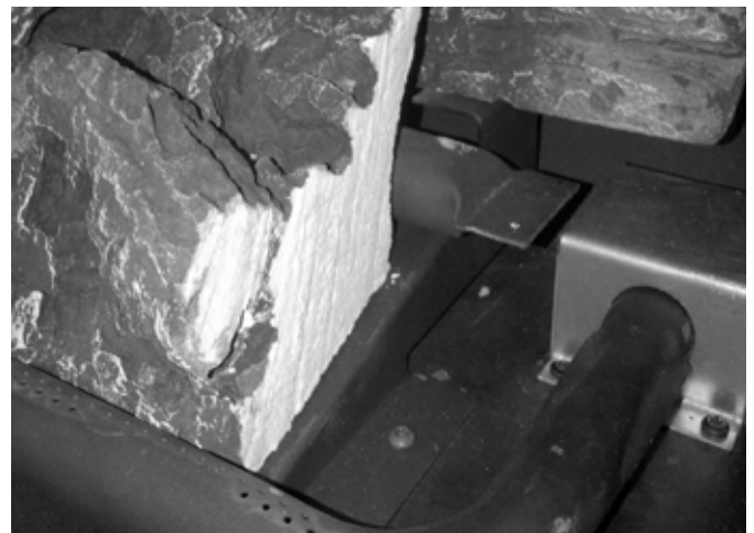
The Ember Bed should sit flat on the support brackets as shown above. *Ember Bed above has been cut for clarity*
