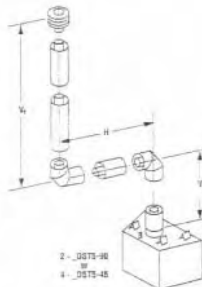
Figure 16 (90° Offsets Shown)
