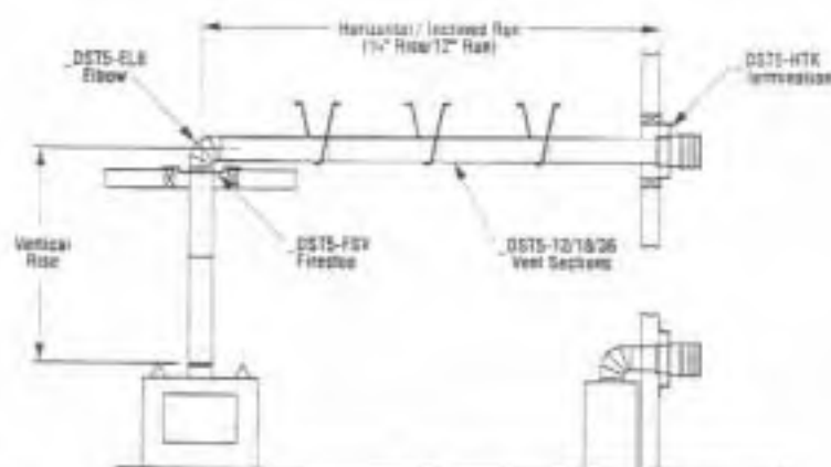
Figure 25 (90° Offsets Shown)
