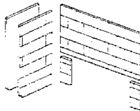
5-Piece Refractory Liner Kit _RLK-38
