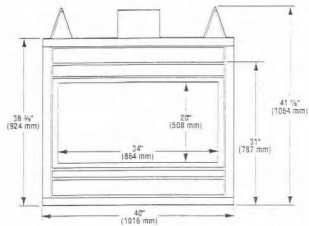
Front View (_DVT6-R)
