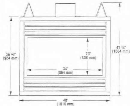
Front View (_DVT6-C)
