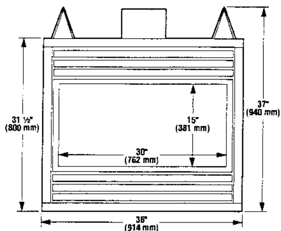
Front View (Model _DVT5-C Shown)
