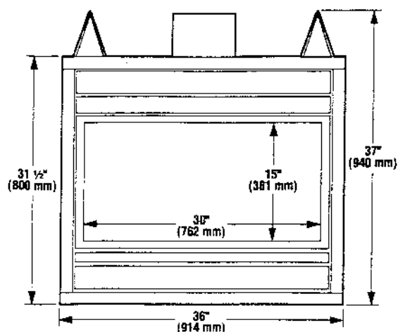
Front View (Model _DVT5-R Shown)
