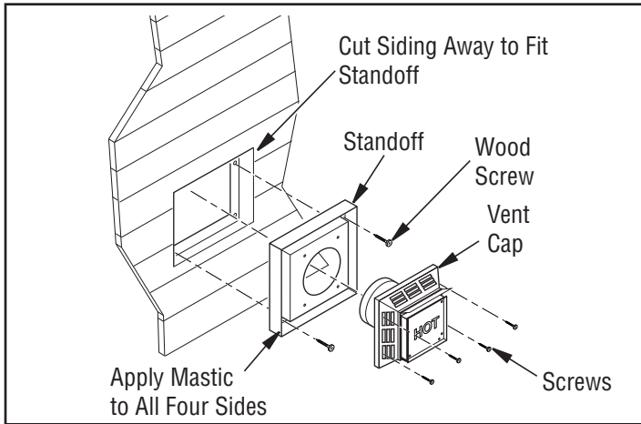
Figure 12 - Installing Siding Standoff (Combustible Exterior Wall)
