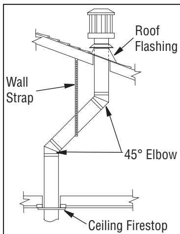
Figure 17 - Offset with Wall Strap and 45° Elbows
