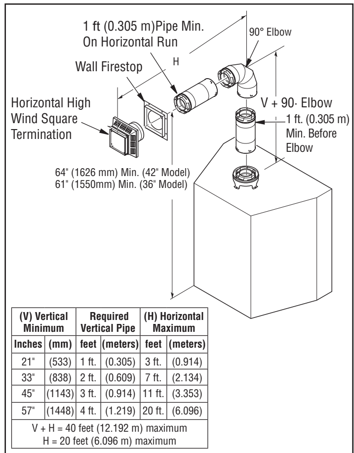
Figure 15 - Horizontal Termination Using One 90° Elbow
