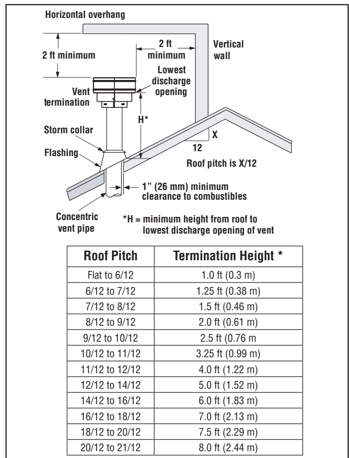
Figure 17a- Termination Heights for Vents above Flat or Sloped Roofs (NFPA 54 / ANSI Z223.1)—Gas Vent Rule
