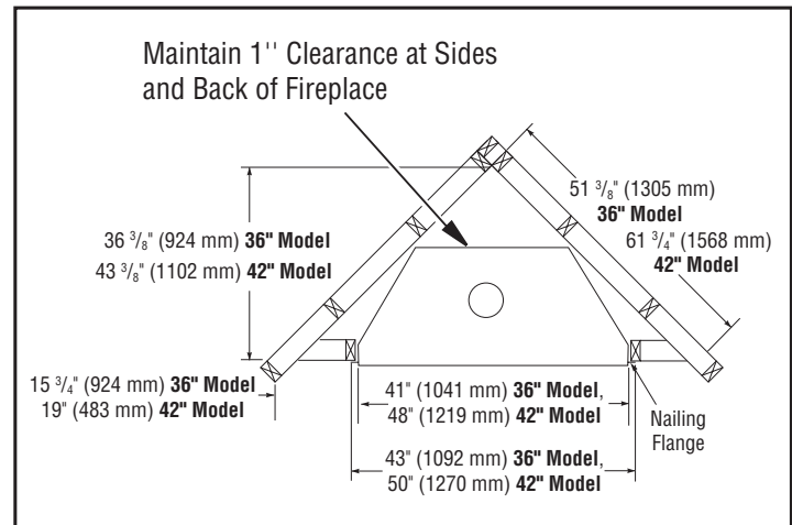
Figure 6 - Framing Clearances for Corner Installation
