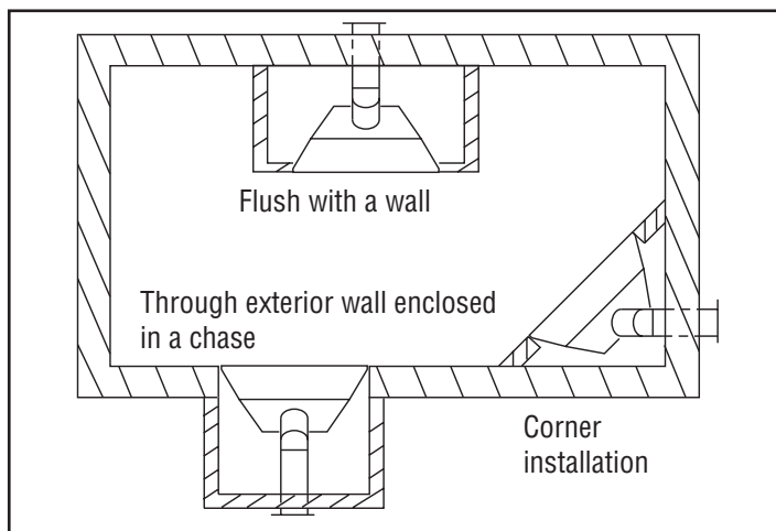
Figure 2 - Common Fireplace Locations
