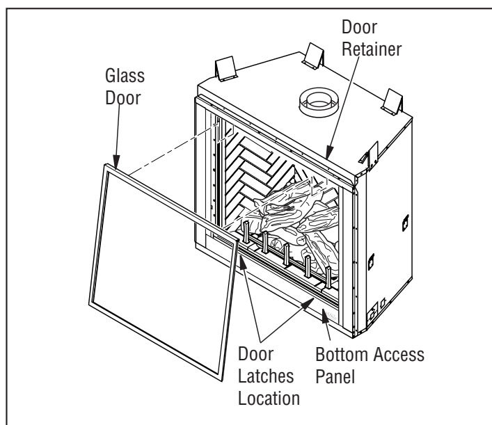
Figure 27 - Removing/Replacing Door
