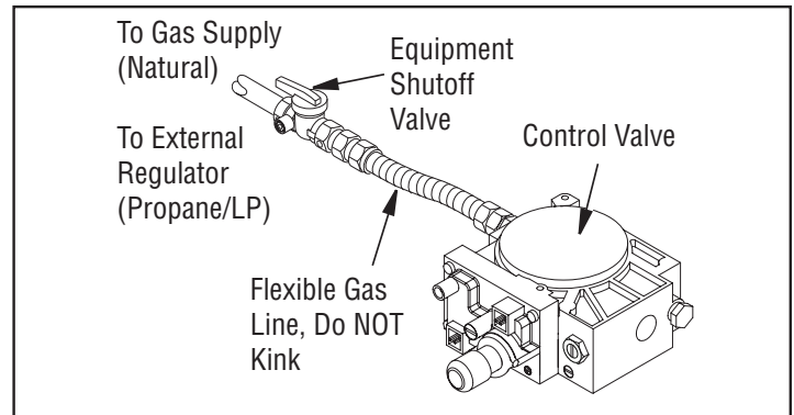
Figure 33 - Connecting/Disconnecting Gas Line to Control Valve
