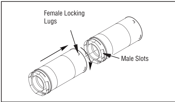
Figure 9 - Vent Pipe Connections
