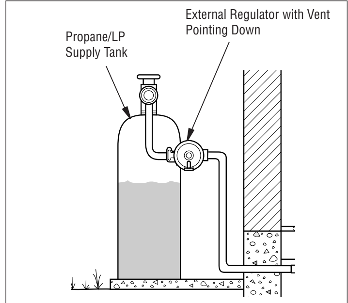
Figure 21 - External Regulator with Vent Pointing Down (Propane/LP Only)
