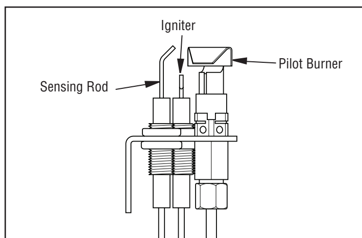
Figure 38 - Pilot
