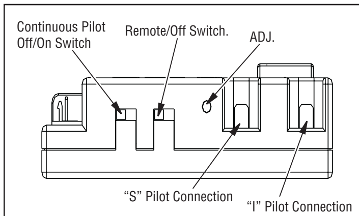
Figure 35 - Gas Module Right Side
