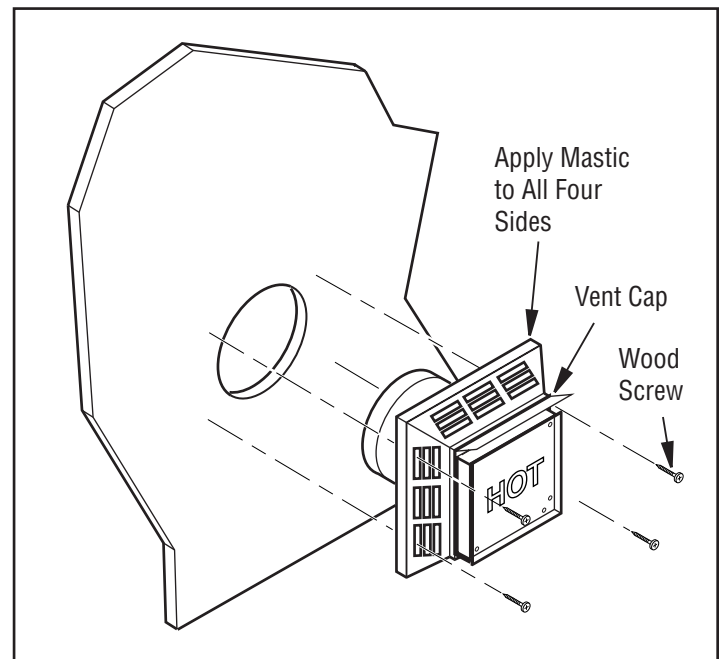
Figure 11 - Installing Horizontal Vent Cap (Noncombustible Exterior)
