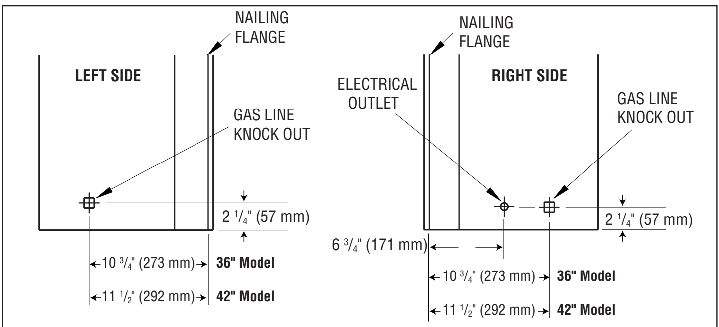
Figure 4 - Electrical Outlet and Gas Knockout Locations
