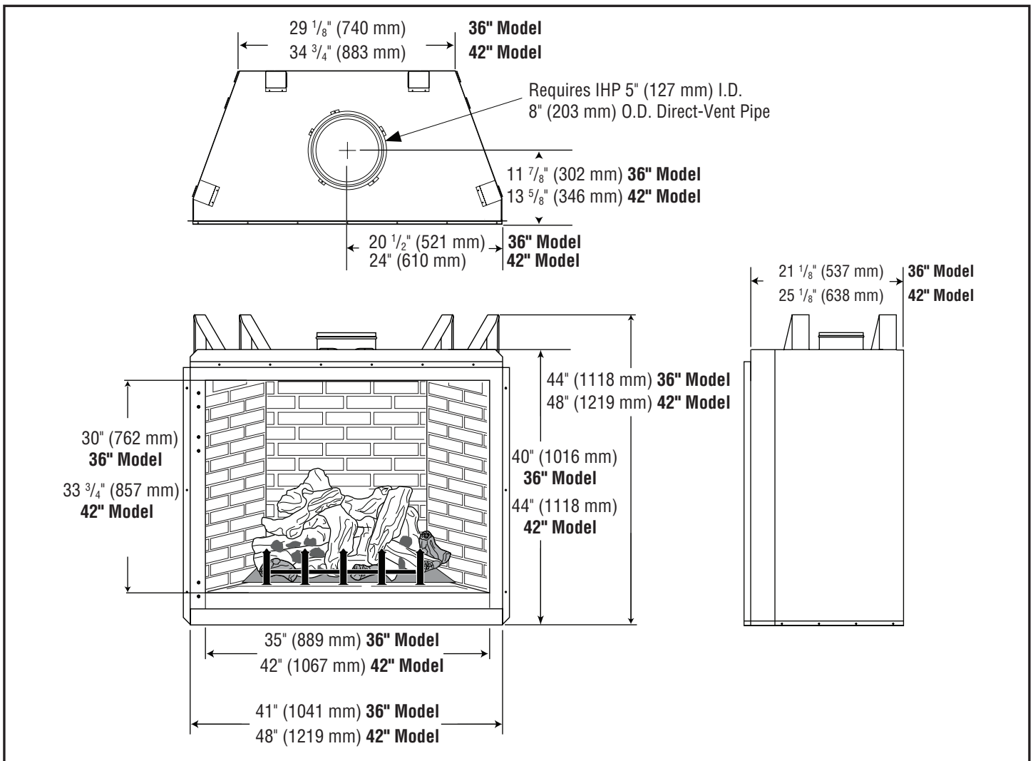
Figure 3 - Fireplace Dimensions
