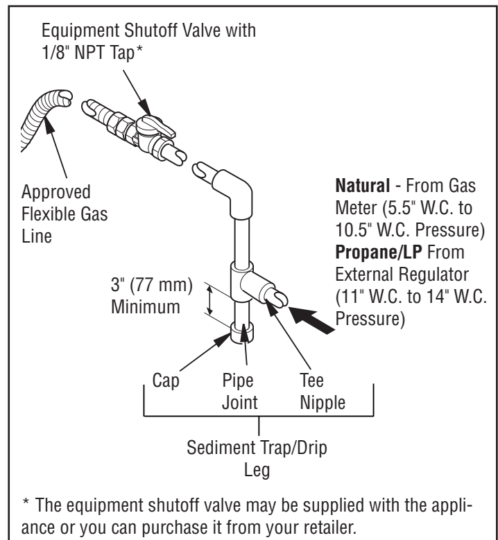
Figure 22 - Gas Connection
