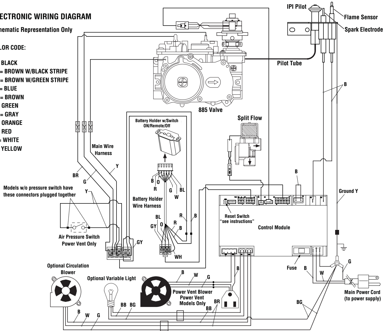
Figure 24 - Electronic Wiring Diagram - SIT Proflame II
