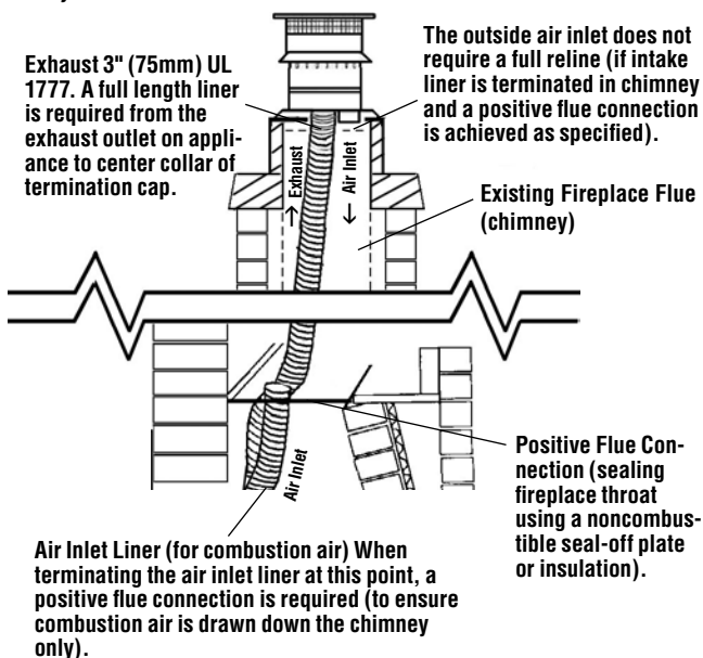
Figure 7a - Terminating Air Inlet in Chimney
