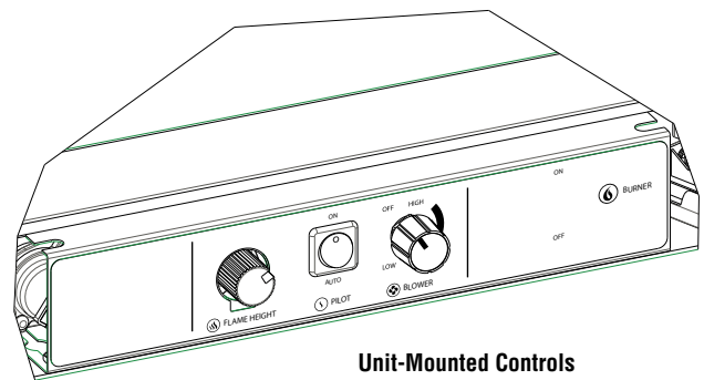
Figure 21A - DRI2530TEN Model
