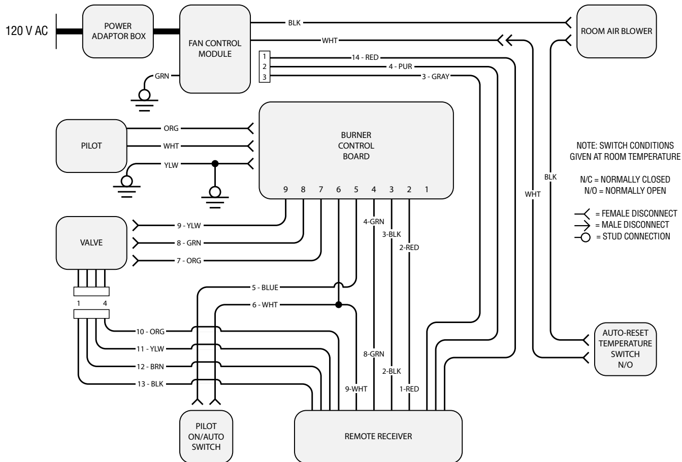
Figure 28C - Electronic Control Schematic - Model DRI3030TEN
